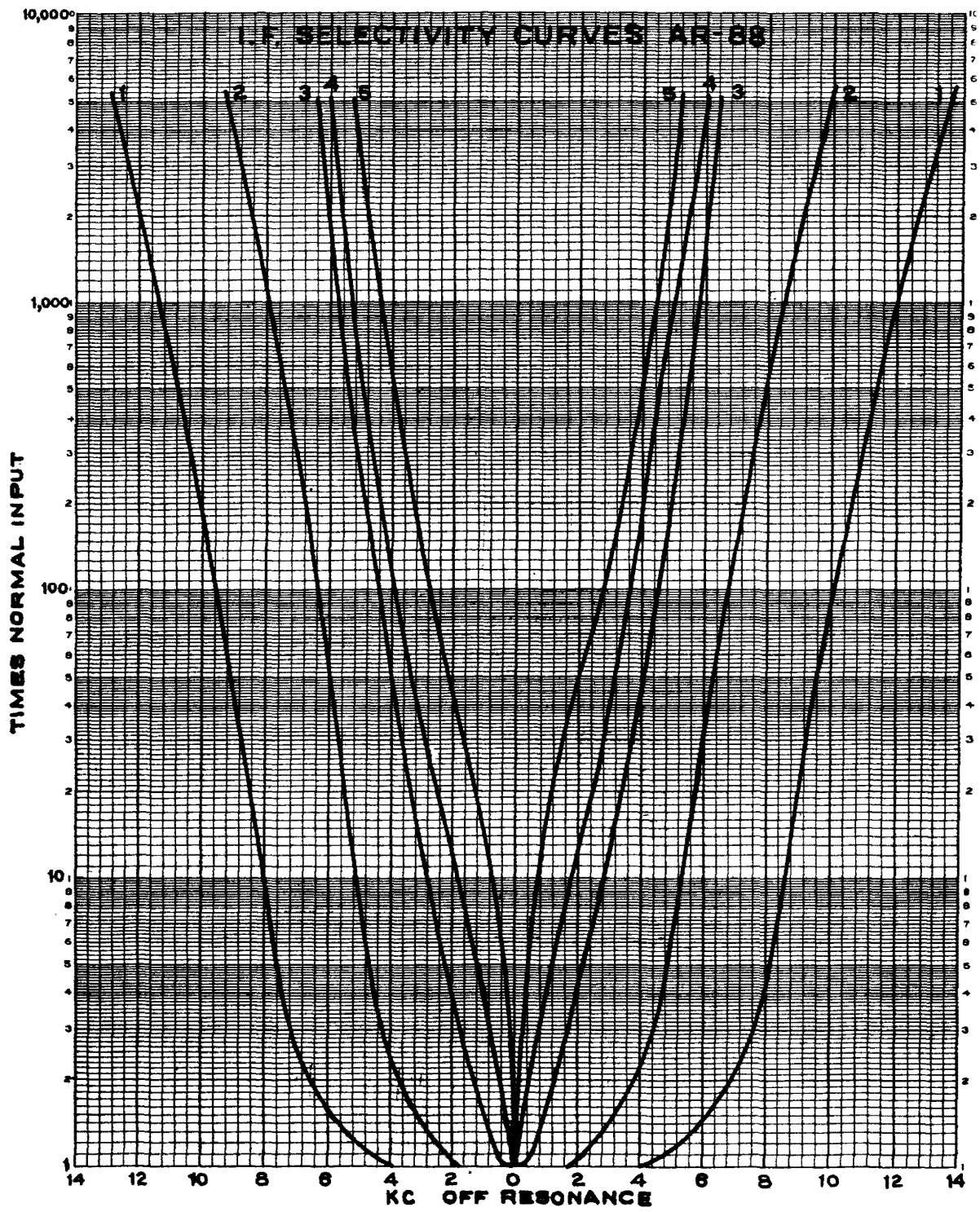
Figure 12—Selectivity Curves
