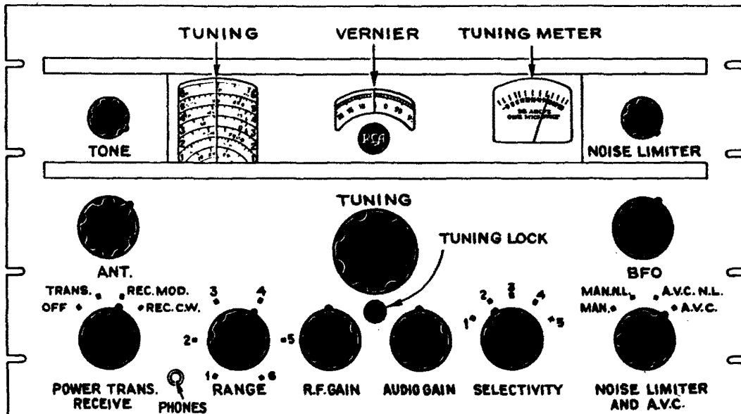
Figure 4—Diagram of Front Panel
