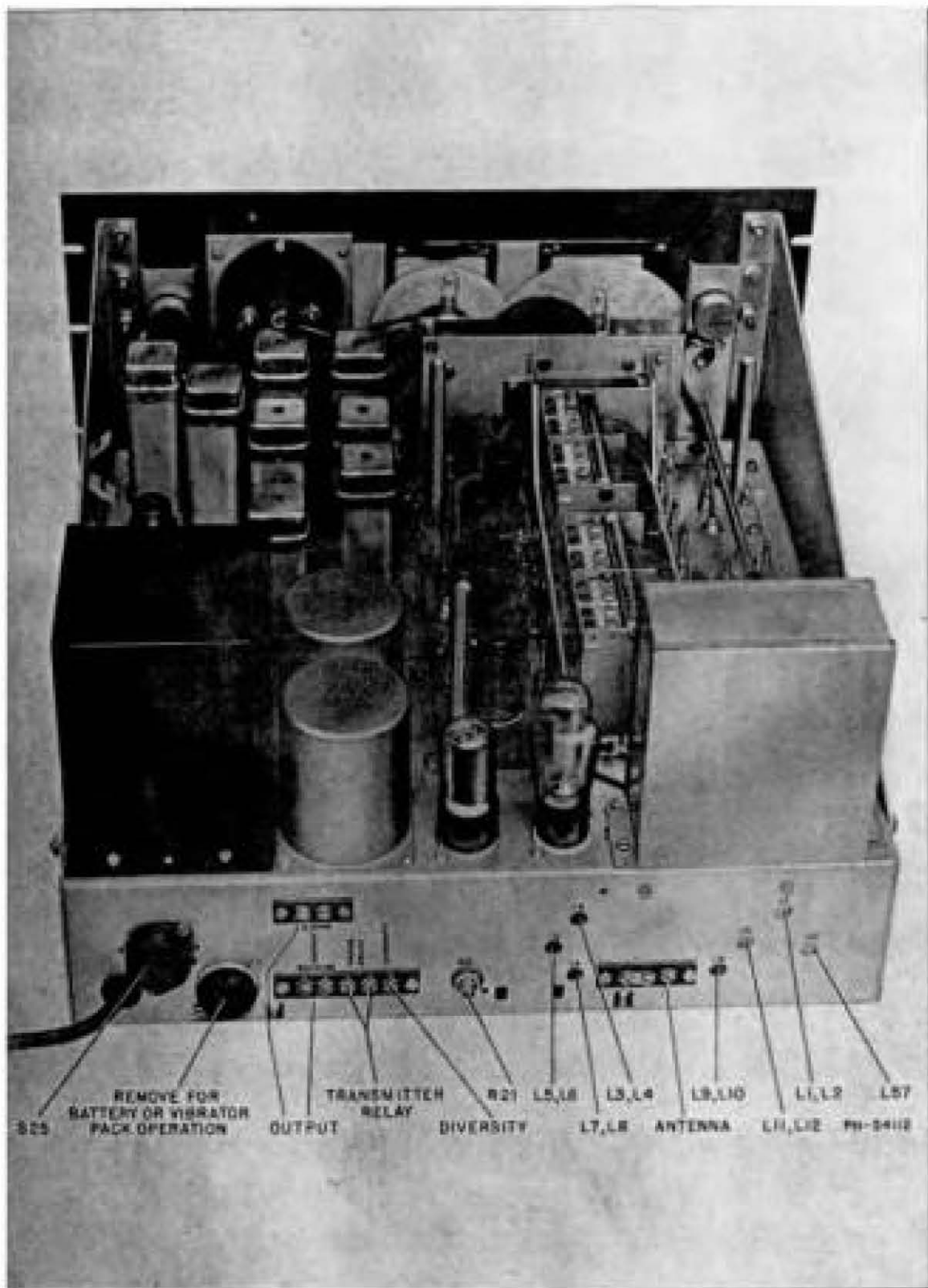
Figure 6—AR-88 Chassis
